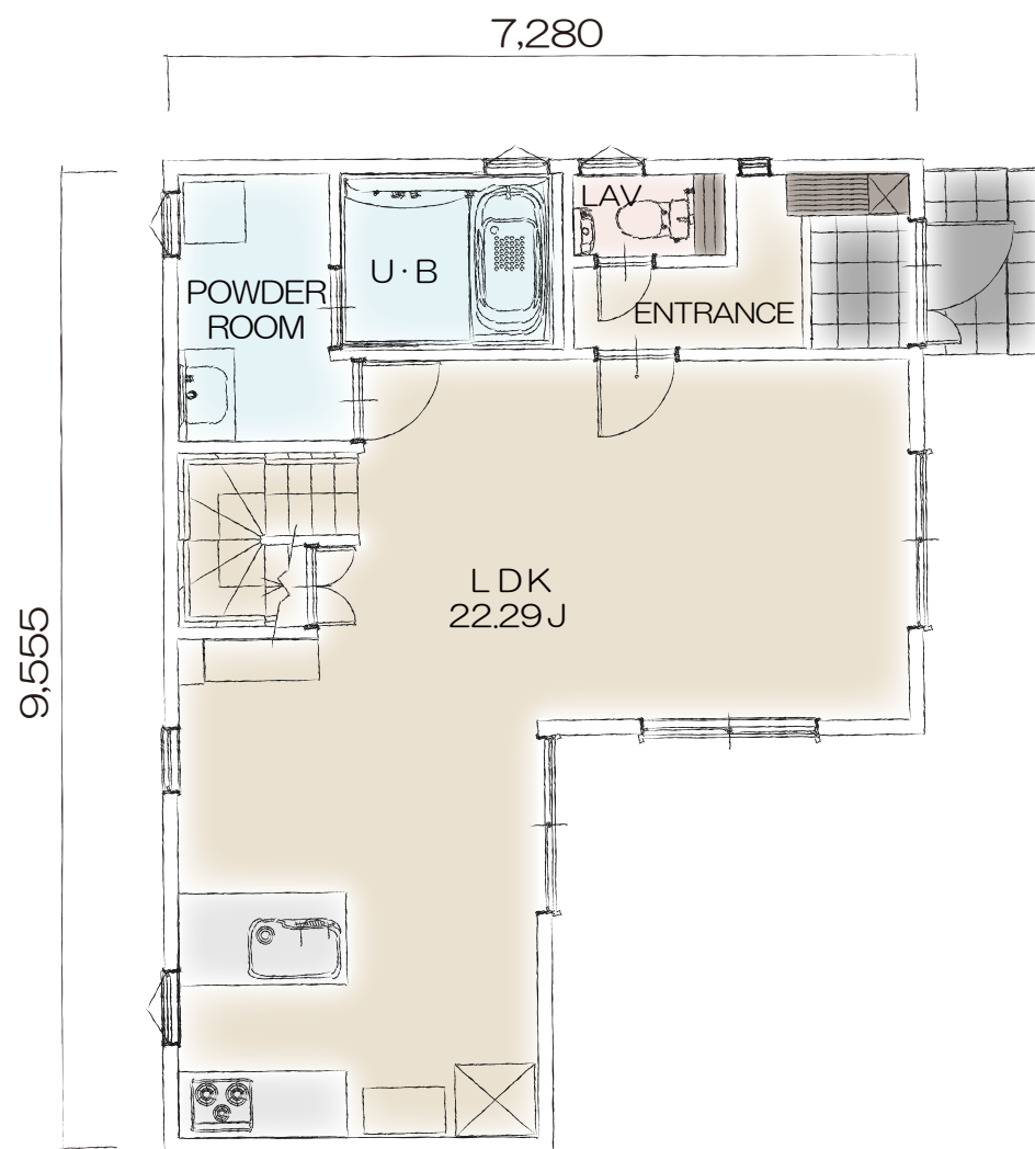
1F PLAN
